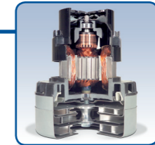
TwinFlo suction motor
